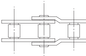
Double offset link
