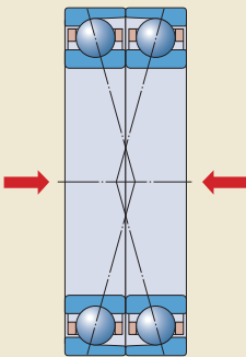
Face-to-face arrangement
