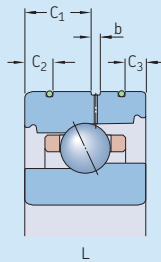
Dimensions for direct oil-air lubrication – 719 .. B and 70 .. B bearing series
