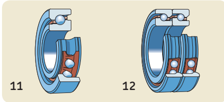
Angular contact thrust ball bearings for screw drives (→ page 337) single direction (BSA and BSD series) (11), universally matchable for mounting as sets (12) – bearings with seals (13) double direction with seals (BEAS series) (14) – for bolt mounting (BEAM series) (15) cartridge units with a flanged housing (FBSA series) (16)
