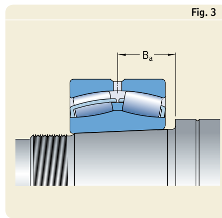
Dimensioning of a tapered journal
