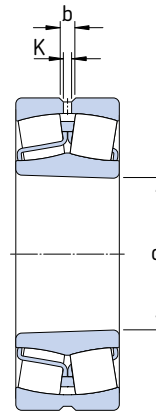
Tapered bored
