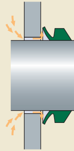
V-ring used as a grease valve
