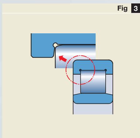
Opened flanges
