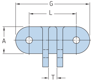
Attachment with flight wings*
