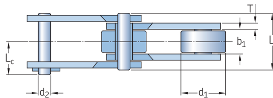
with large rollers
