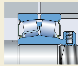
KMFE lock nut
