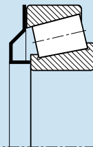
JV -An internally sealing NILOS-Ring for a single-row tapered roller bearing would be designated type 302 07 JV.
