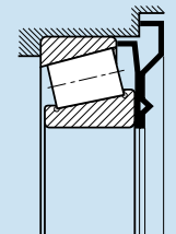
AK -A double externally sealing NILOS-Ring for a single-row tapered roller bearing would be designated type 313 11 AK.
