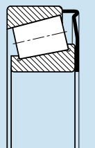
AV -An externally sealing NILOS-Ring for a single-row tapered roller bearing would be designated type 302 07 AV.
