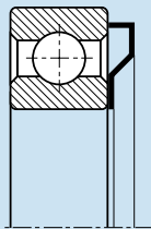
AV -An externally sealing NILOS-Ring for a single-row deep-groove ball bearing would be designated type 6410 AV.
