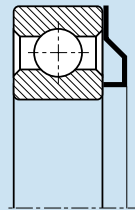
JV -An internally sealing NILOS-Ring for a single-row deep-groove ball bearing would be designated type 6410 JV.
